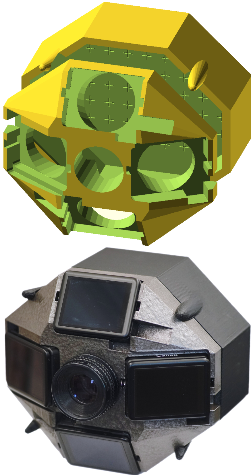
Figure 3. 3D-Printed Multi-Camera Frame Design And Prototype
