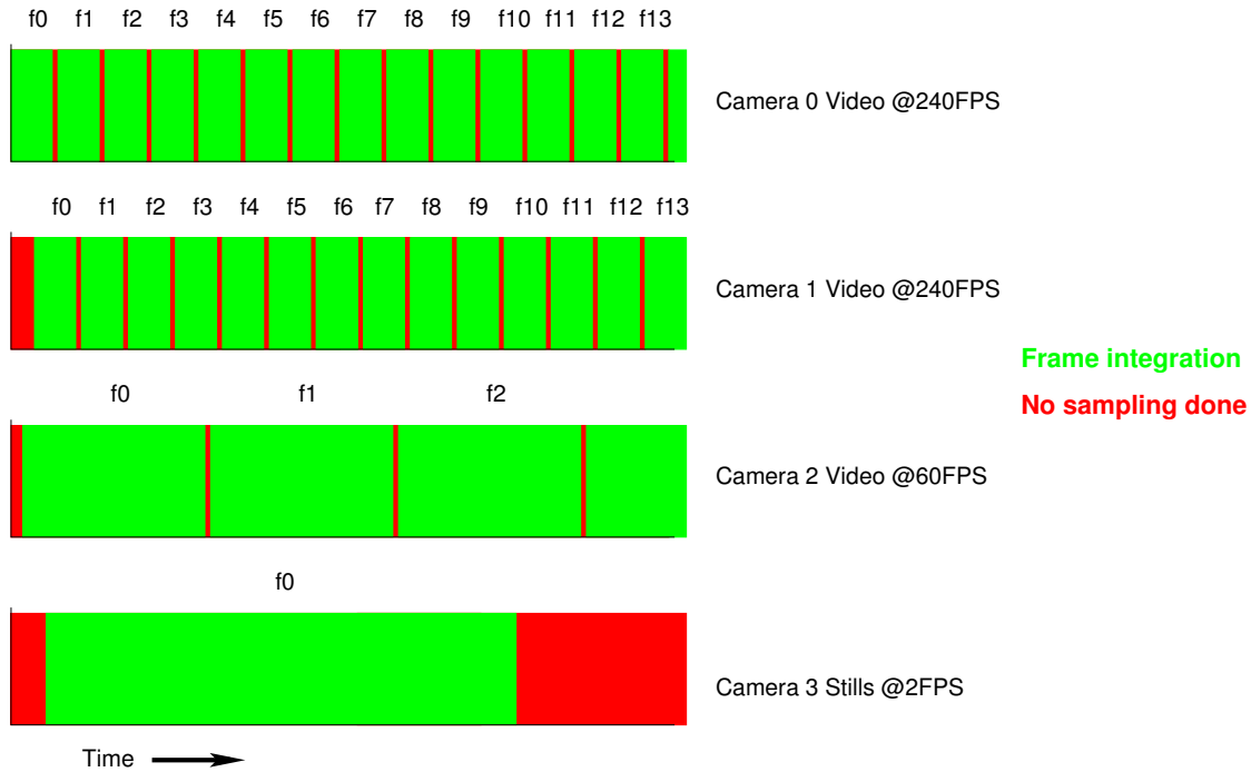
Figure 5. Overview Of Multi-Camera Control
